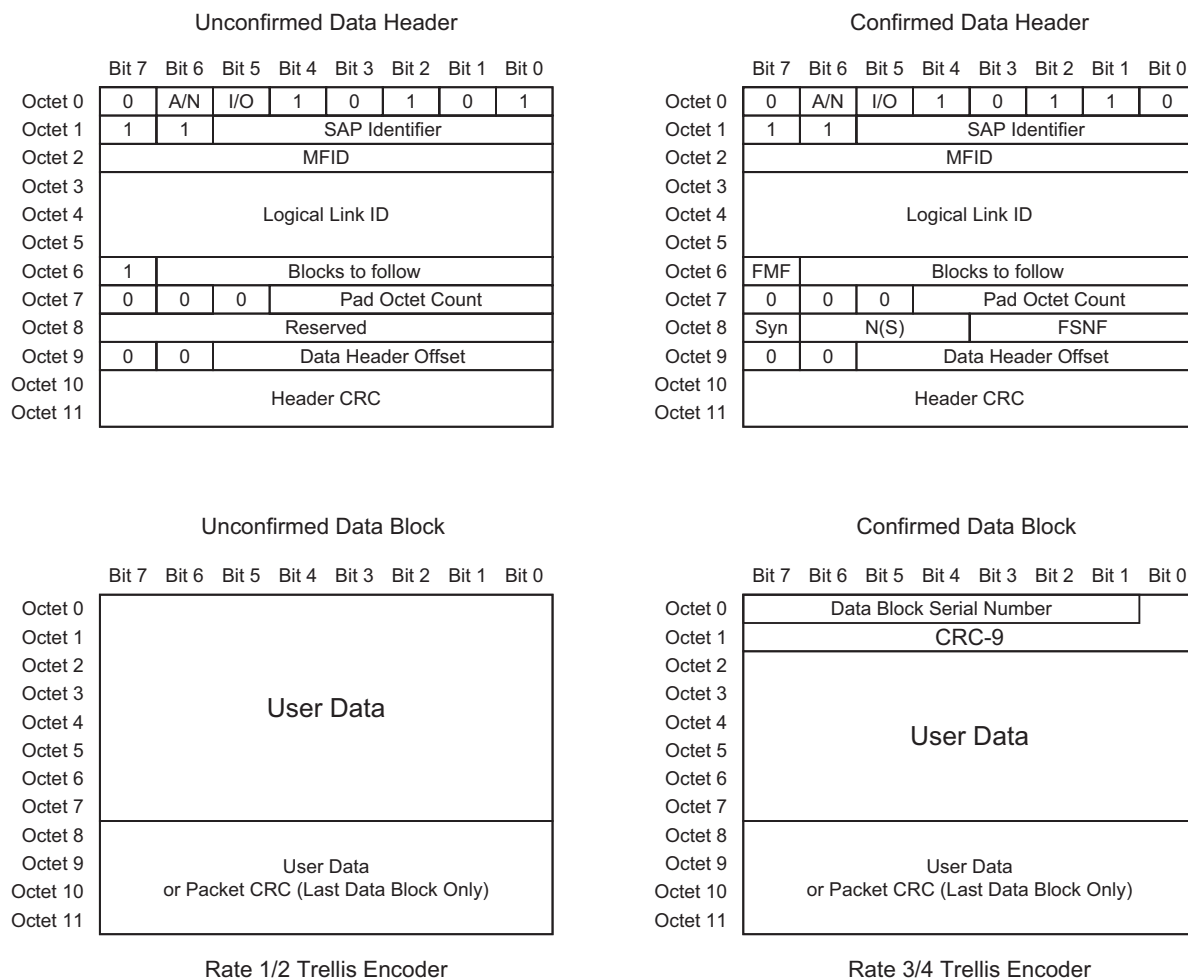
Rate 1/2 Trellis Encoder
