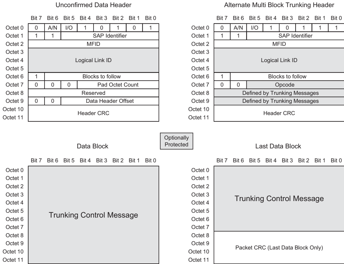
Figure 6-7: Multiple Block Trunking (MBT)
