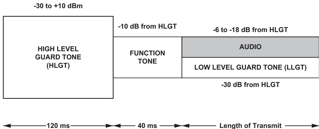
Figure 5-3: Tone Remote Control Sequence
