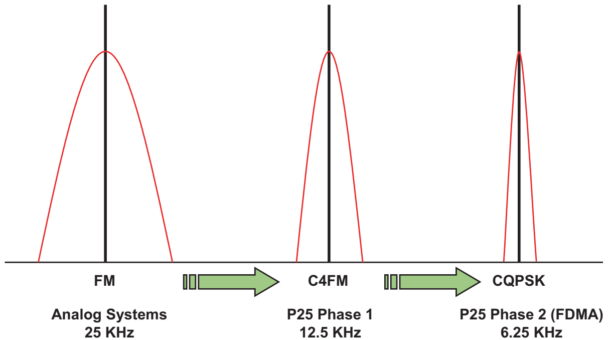
Figure 1-6: P25 Spectrum Efficiency
