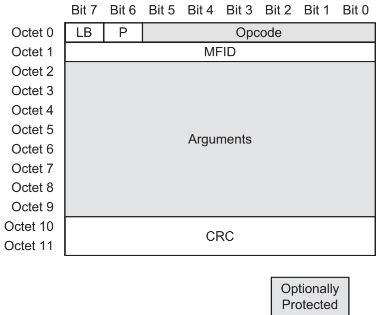
Figure 6-5: Trunking Signaling Block (TSBK)
