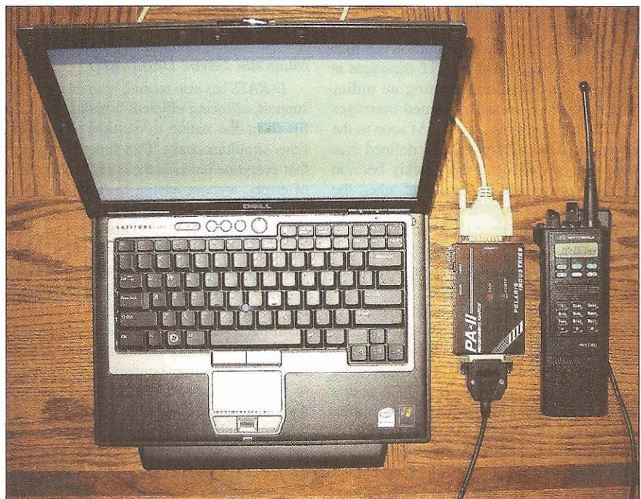
To reprogram a Motorola Astro Saber, you need Motorola's programming software, a Radio Interface Box (RIB) and the appropriate cables. You can find the RIB and cables on eBay and other sites.
