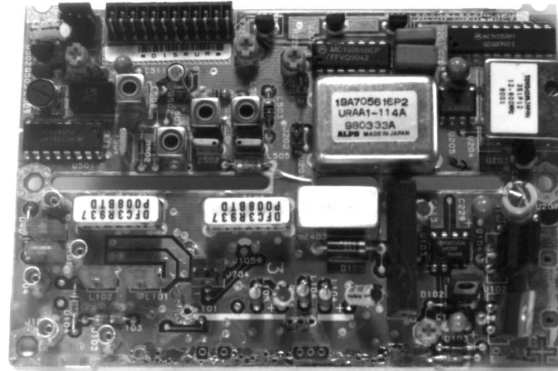
19D902132G3 RF Board 25W 19D902132G4 RF Board 15W (Shown)
