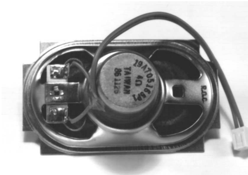
19A705165P1 Speaker
