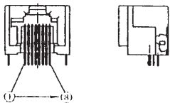
8P MODULAR CONNECTOR PIN NO.
