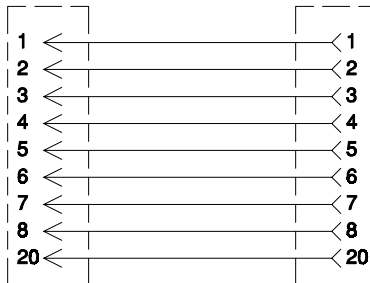
CONNECTOR #1
