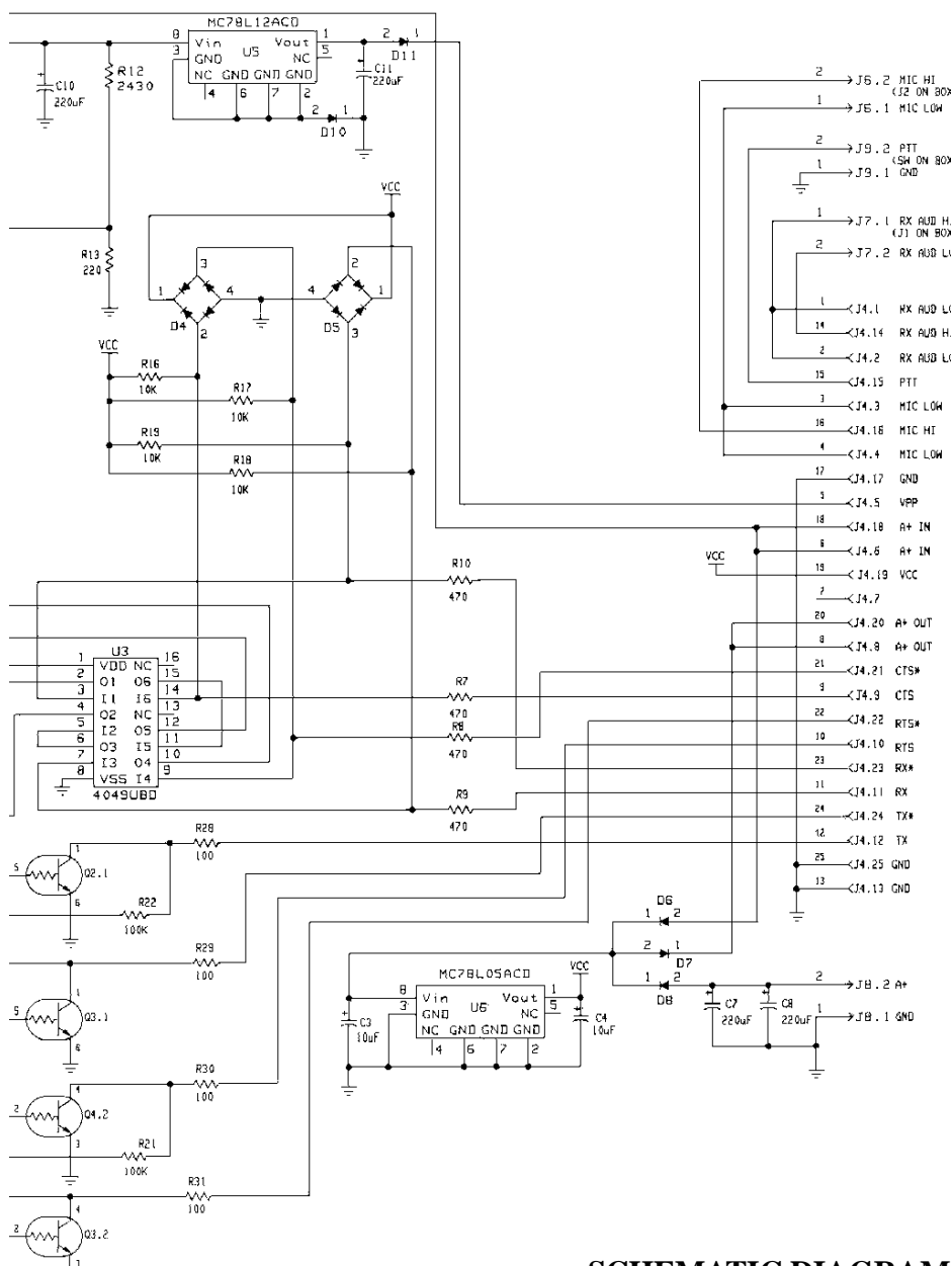
SCHEMATIC DIAGRAM Circuit Board A1 19D904011G1
