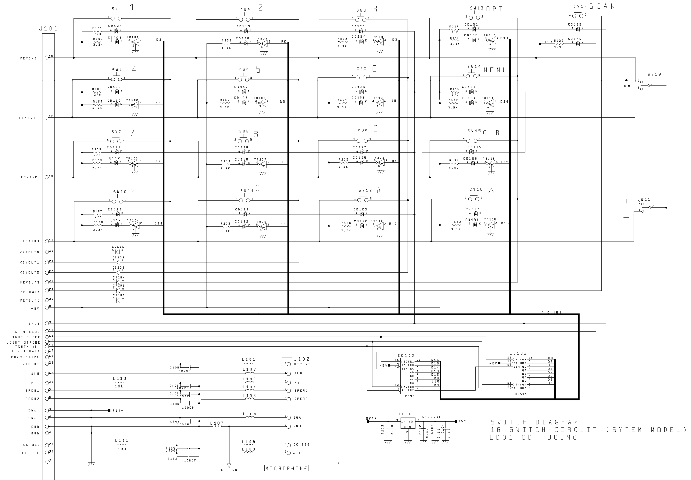
SCHEMATIC DIAGRAM Switch Circuit (System Model) ED01-CDF-368MC
