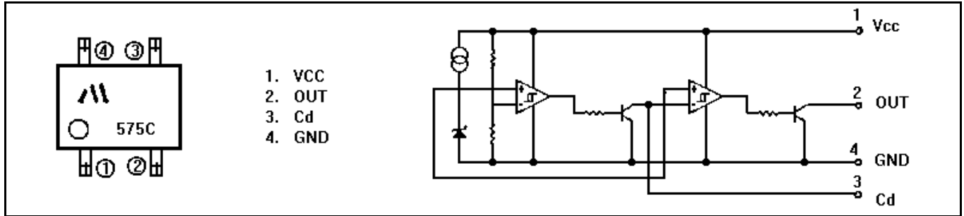
Figure 7-8: IC206 System Reset (PST575CMT)
