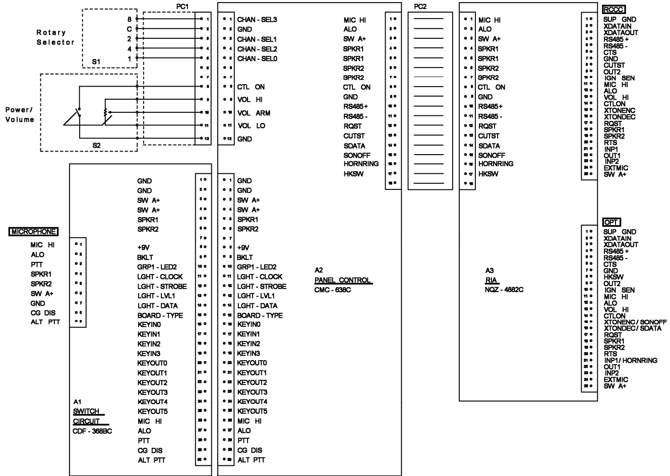
Figure 13-2: Control Unit (Scan Remote) (ED00-CMD-556BRC)
