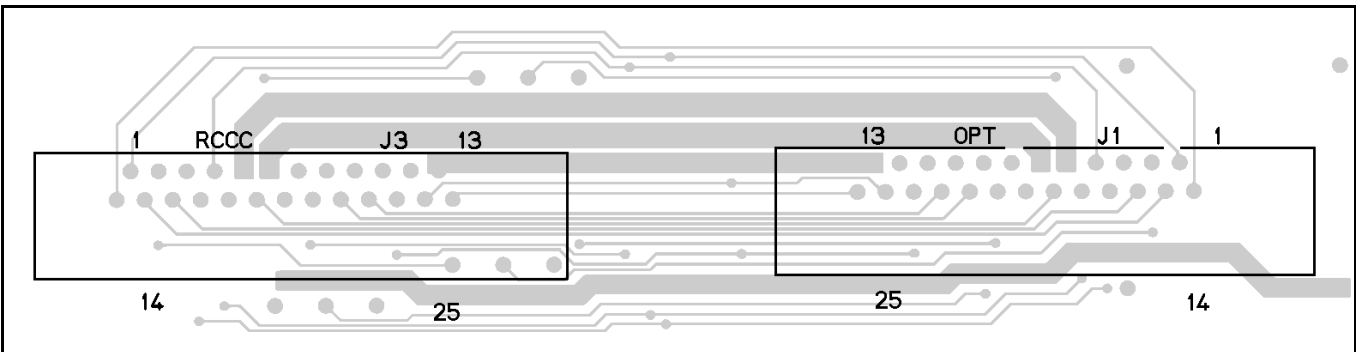
Figure 8-3: Remote Interface Adaptor NQZ-4882C Component Side
