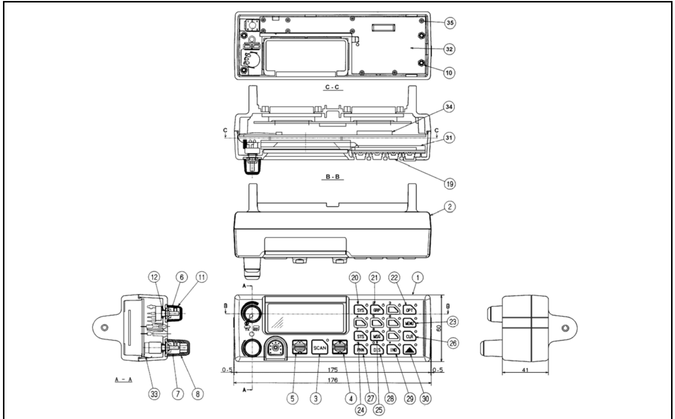
Figure 10-4: Remote System Model KRY 101 1632/14 (CMC-556 MRC, Sh. 2)
