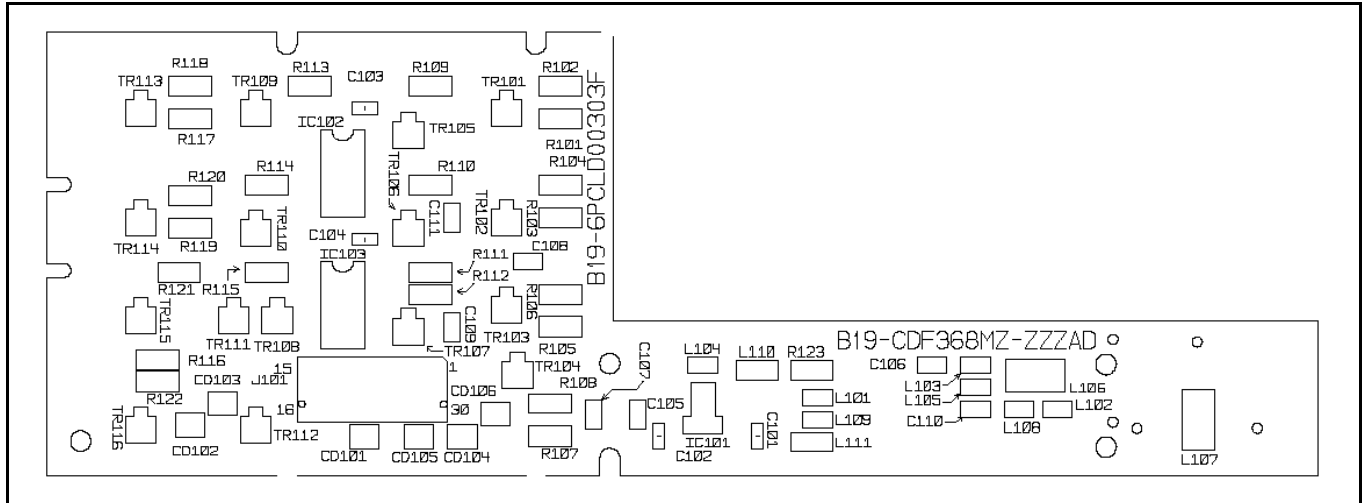
Figure 8-5: Switch Circuit CDF-368MC Component Side
