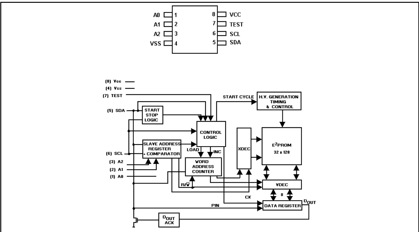
Figure 7-4: IC202 EEPROM (AT24C04N-10SI)
