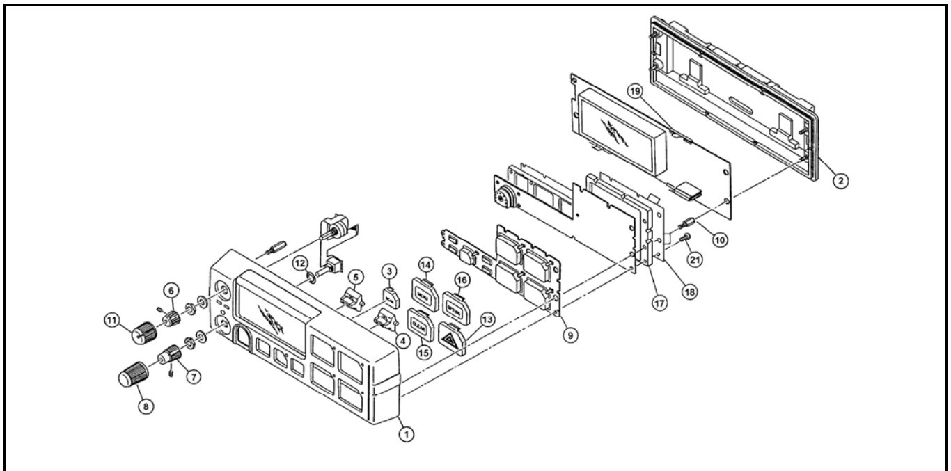
Figure 10-8: Local Scan Model KRY 101 1632/11 & KRY 101 1632/17 (CMC-556 BLC, Sh. 1)
