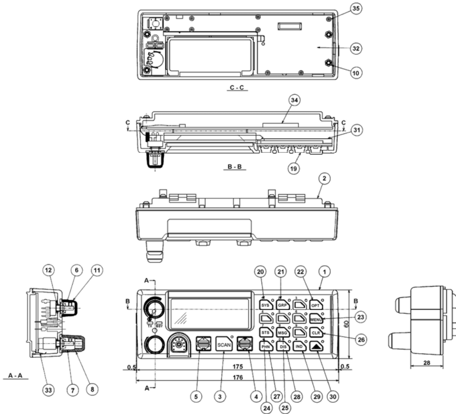
Figure 10-10: Local System Model KRY 101 1632/13 & KRY 101 1632/19 (CMC-556 MLC, Sh. 2)
