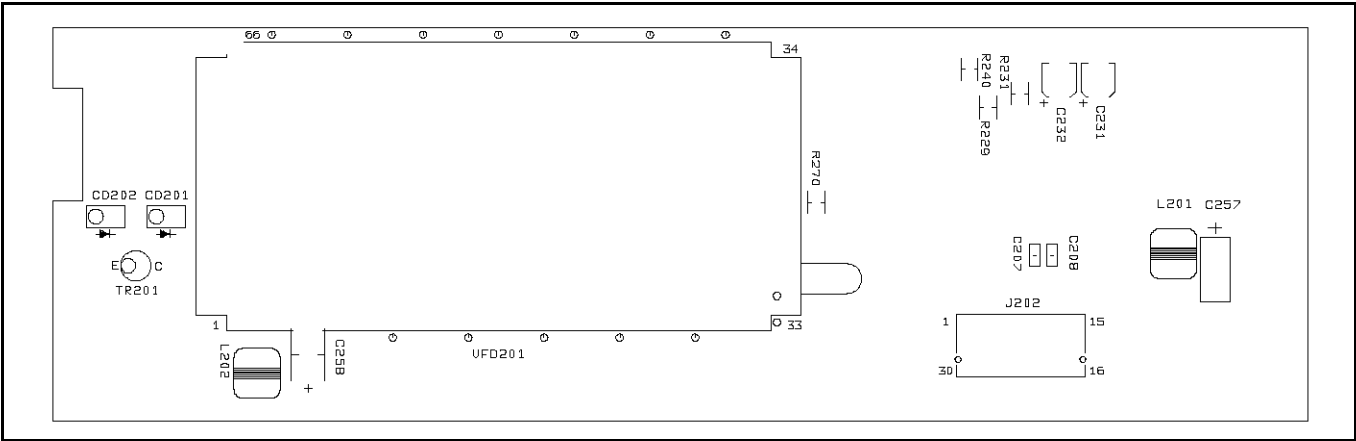
Figure 8-2: Panel Control CMC-638C Solder Side
