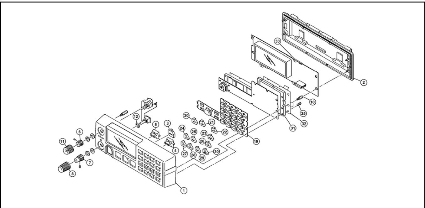
Figure 10-11: Local System Model KRY 101 1632/13 & KRY 101 1632/19 (CMC-556 MLC, Sh. 1)
