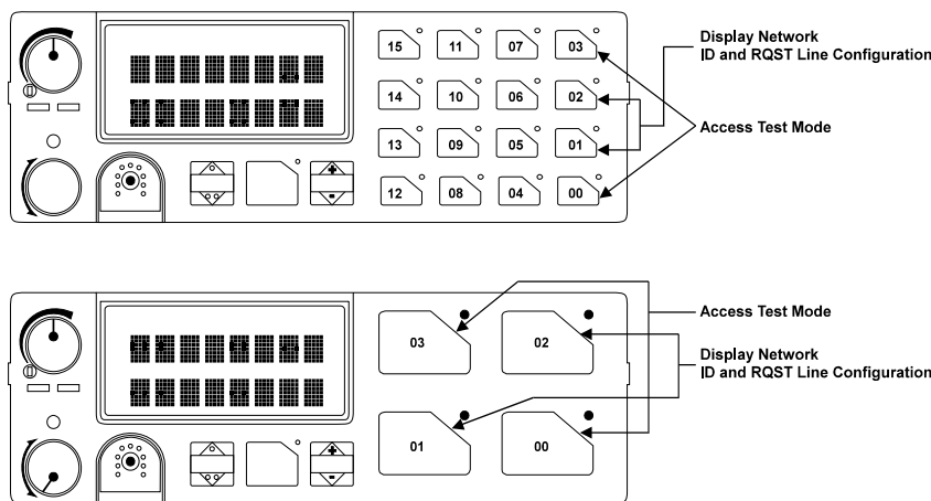
Figure 5-1: Access Control Unit Test Mode
