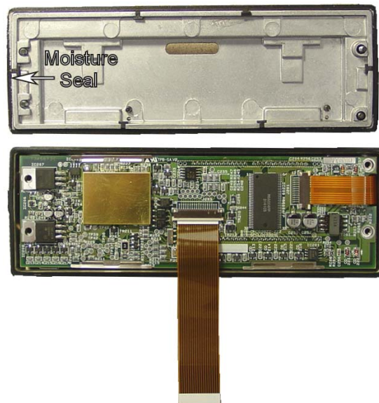
Figure 4-10: Orion Control Unit
