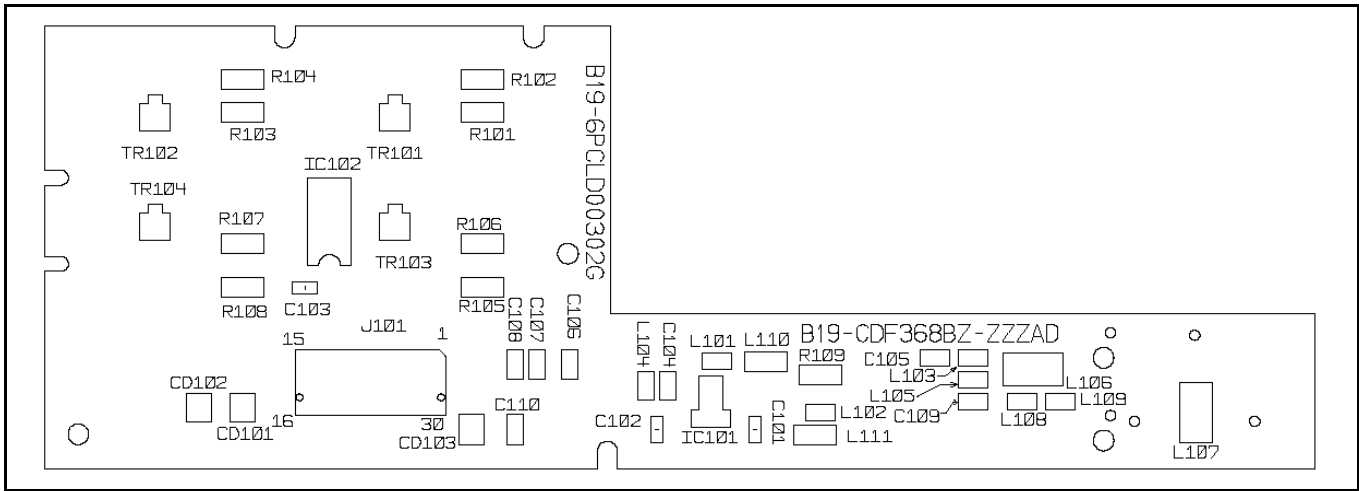
Figure 8-7: Switch Circuit CDF-368BC Component Side
