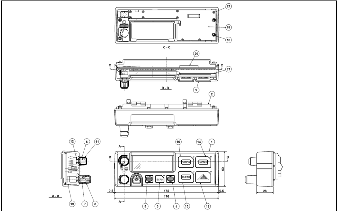
Figure 10-7: Local Scan Model KRY 101 1632/11 & KRY 101 1632/17 (CMC-556 BLC, Sh. 2)
