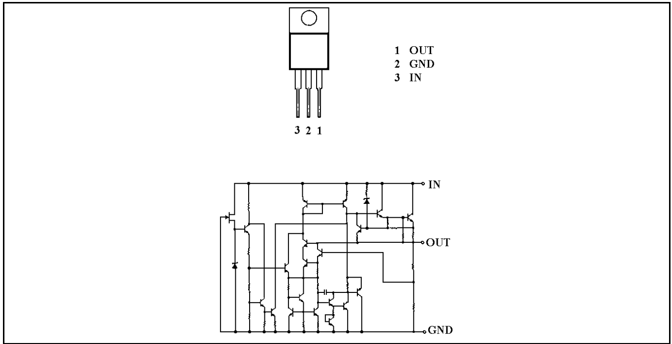
Figure 7-9: IC207 Positive Voltage Regulator (NJM7805A)
