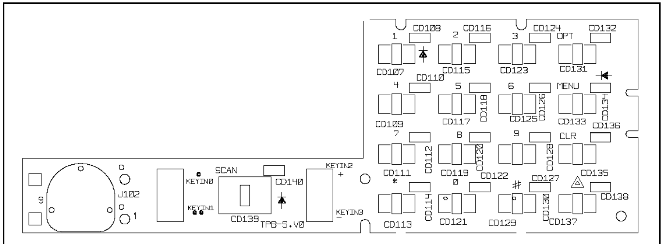
Figure 8-6: Switch Circuit CDF-368MC Solder Side
