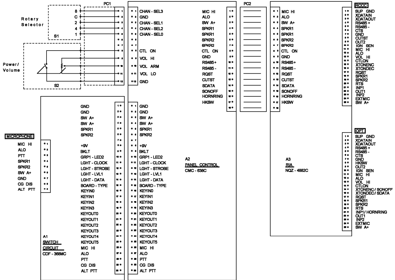
Figure 13-4: Control Unit (System Remote) (ED00-CMD-556MRC)
