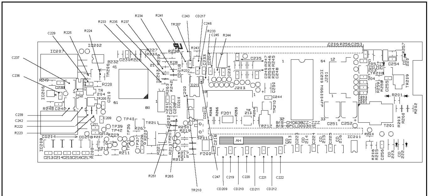
Figure 8-1: Panel Control CMC-638C Component Side
