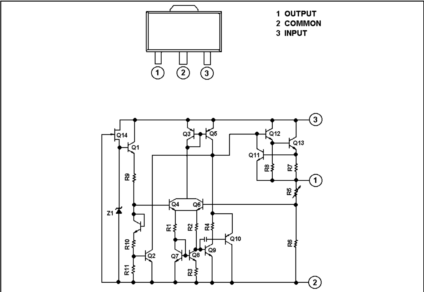
Figure 7-1: IC101 Positive Voltage Regulator (TA78L05F)
