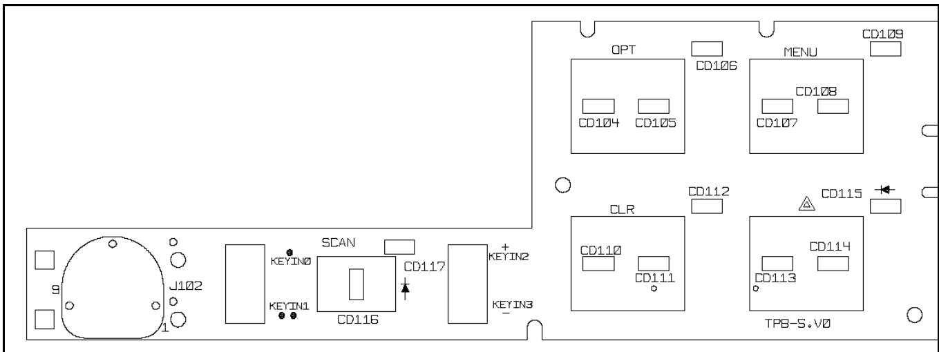
Figure 8-8: Switch Circuit CDF-368BC Solder Side
