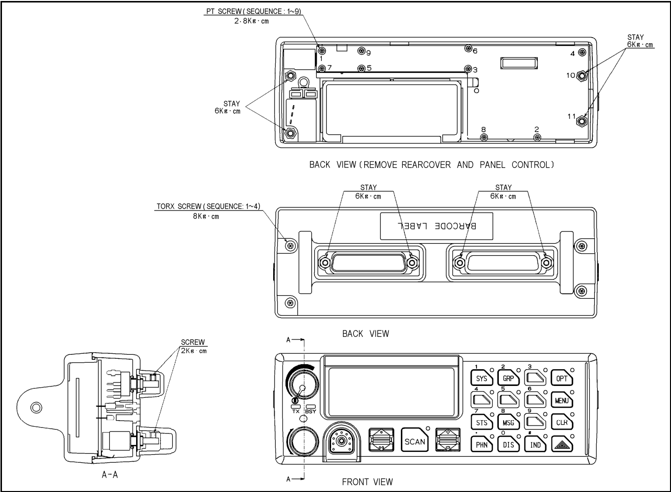
Figure 10-6: Remote System Model KRY 101 1632/14 (CMC-556 MRC, Sh. 3)
