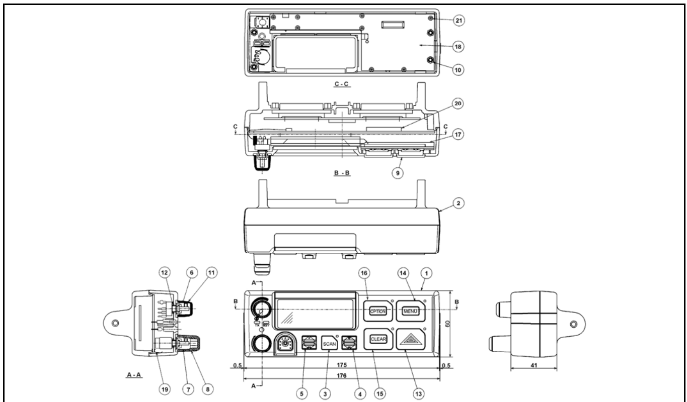
Figure 10-1: Remote Scan Model KRY 101 1632/12 (CMC-556 BRC, Sh. 2)
