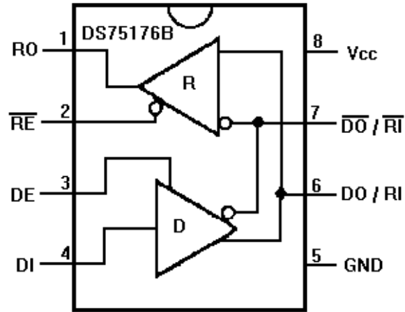
Figure 7-6: IC204 RS-485 Transceiver (DS75176BM)
