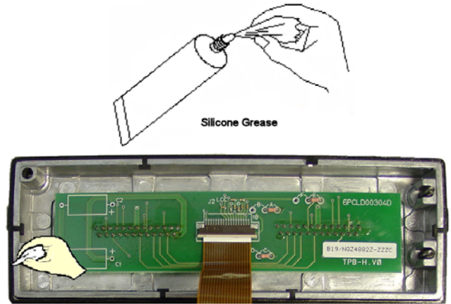
Figure 4-13: Local (Front Mount) Control Unit
