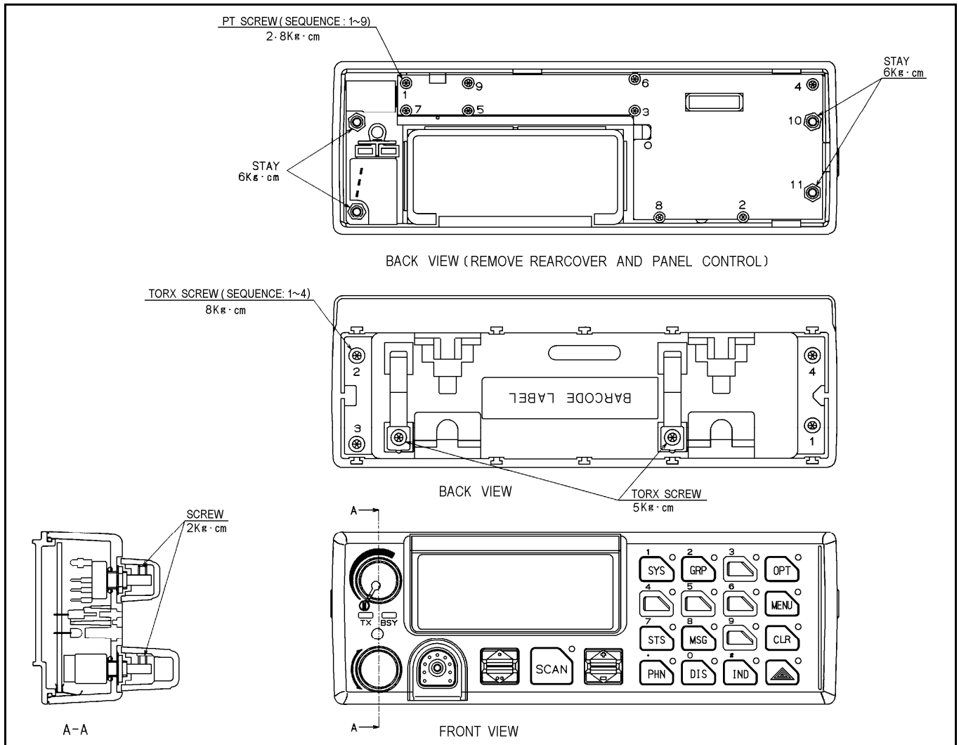
Figure 10-12: Local System Model KRY 101 1632/13 & KRY 101 1632/19 (CMC-556 MLC, Sh. 3)
