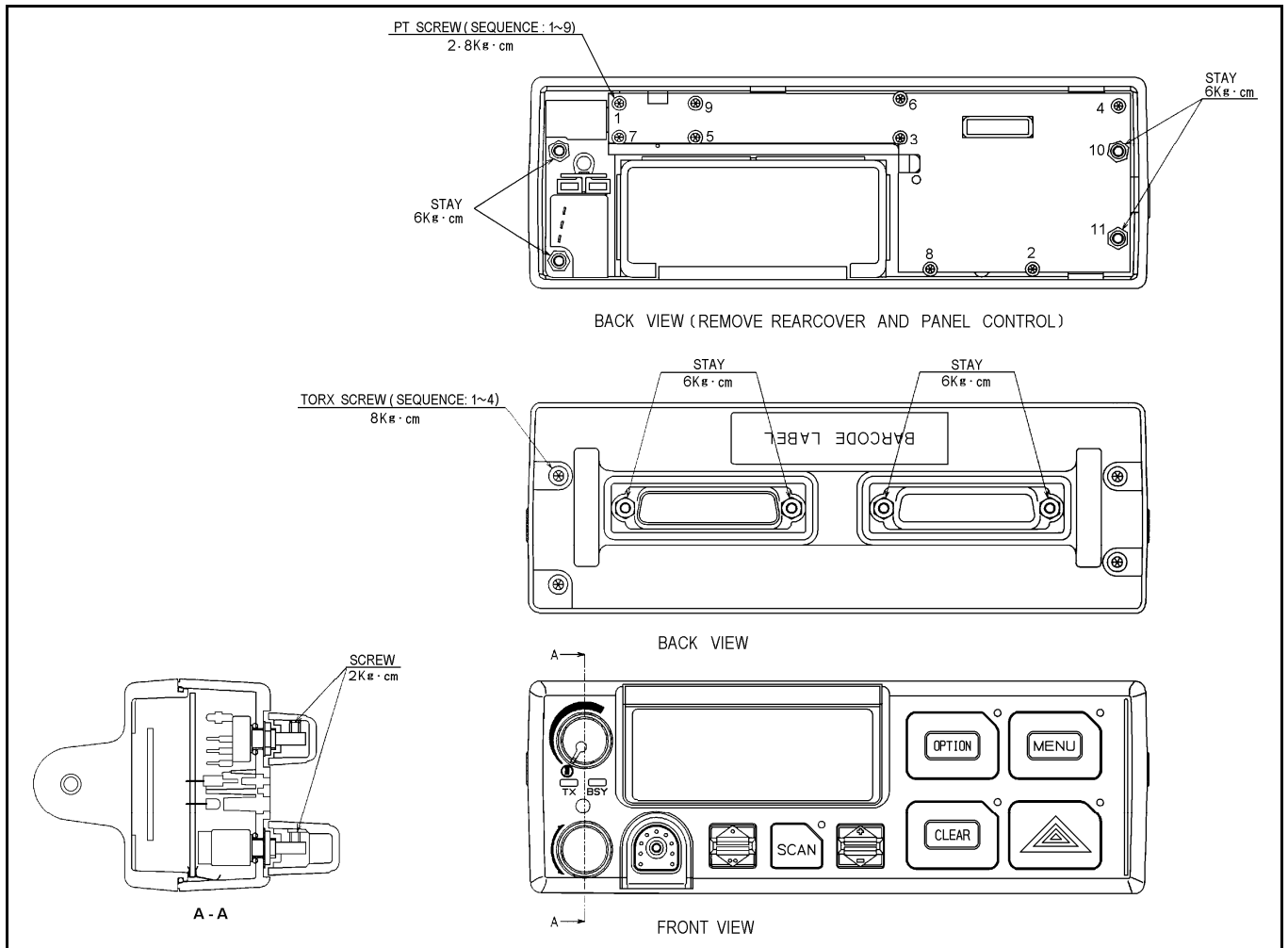
Figure 10-3: Remote Scan Model KRY 101 1632/12 CMC-556 BRC, Sh. 3)
