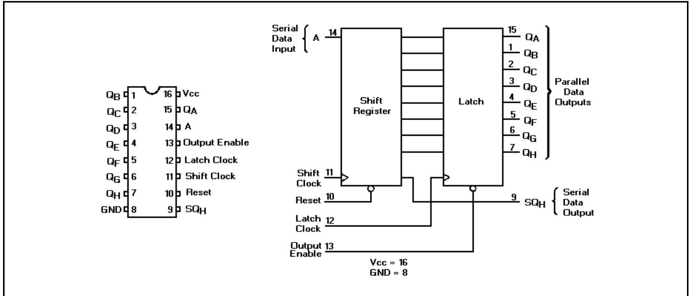
Figure 7-2: IC102 8 Bit Shift Register (MC74HC595AF)
