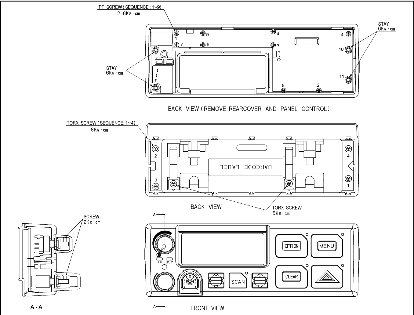
Figure 10-9: Local Scan Model KRY 101 1632/11 & KRY 101 1632/17 (CMC-556 BLC, Sh. 3)
