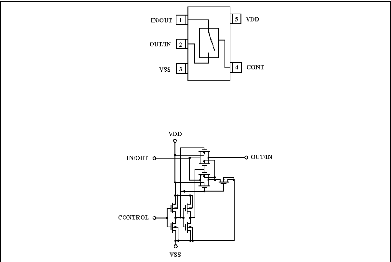
Figure 7-7: IC205 Bilateral Switch (SC14S66F)
