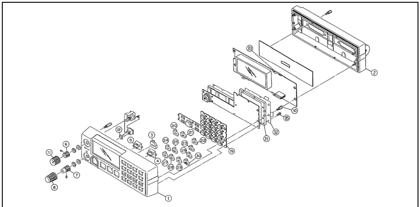
Figure 10-5: Remote System Model KRY 101 1632/14 (CMC-556 MRC, Sh. 1)
