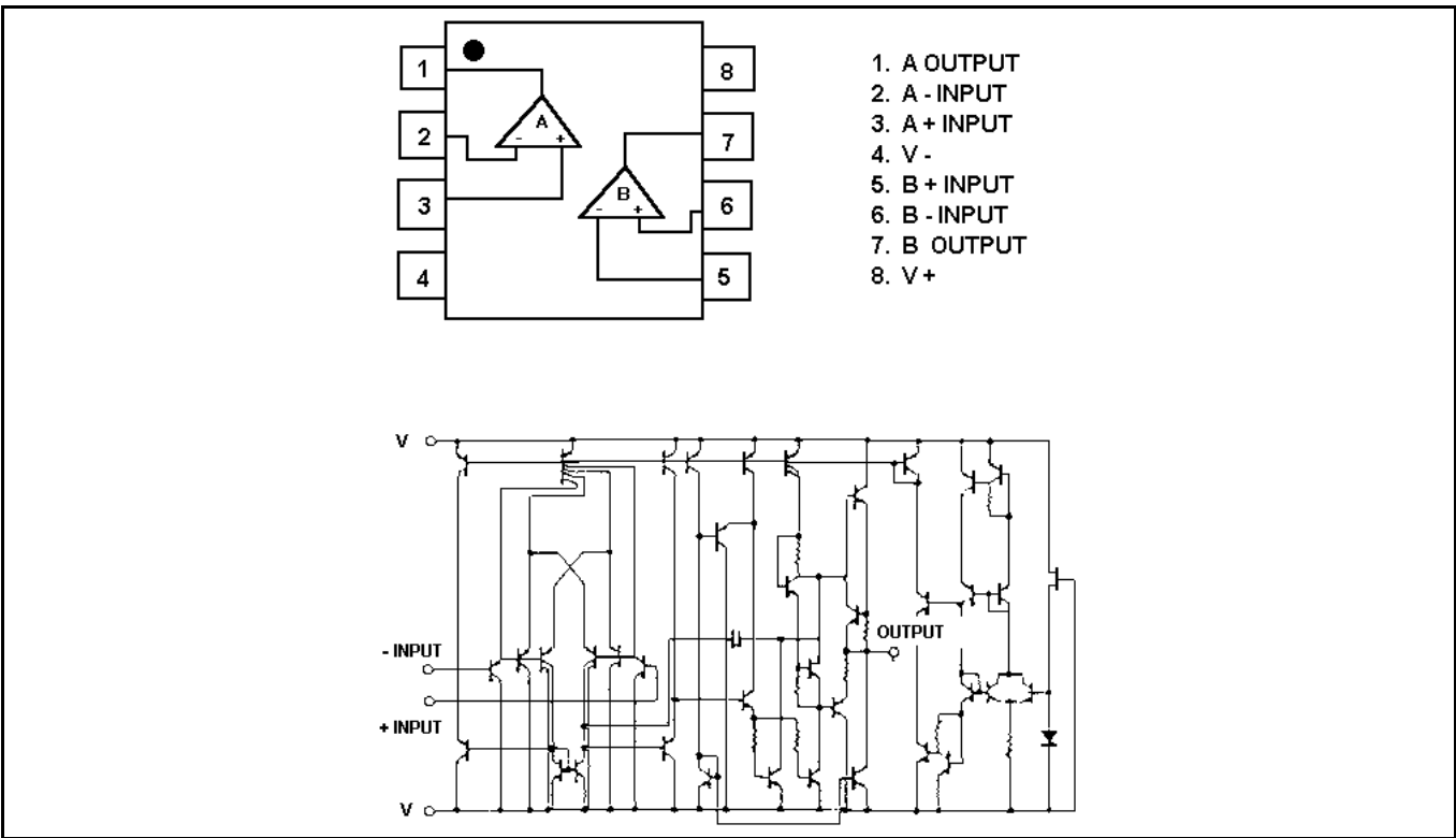
Figure 7-3: IC201 Dual Operational Amplifier (NJM3404M)
