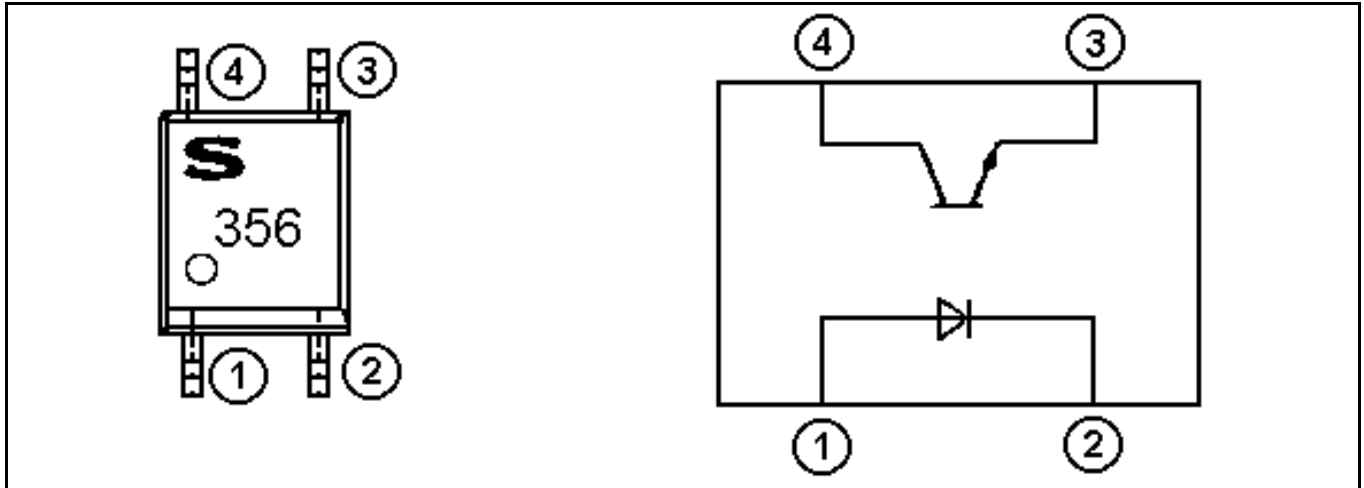
Figure 7-12: IC210, 211 Photocoupler (PC356T)
