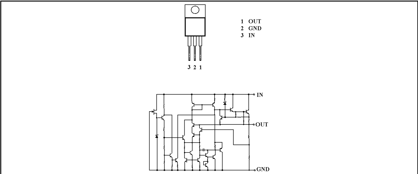
Figure 7-10: IC208 Positive Voltage Regulator (NJM7809A)
