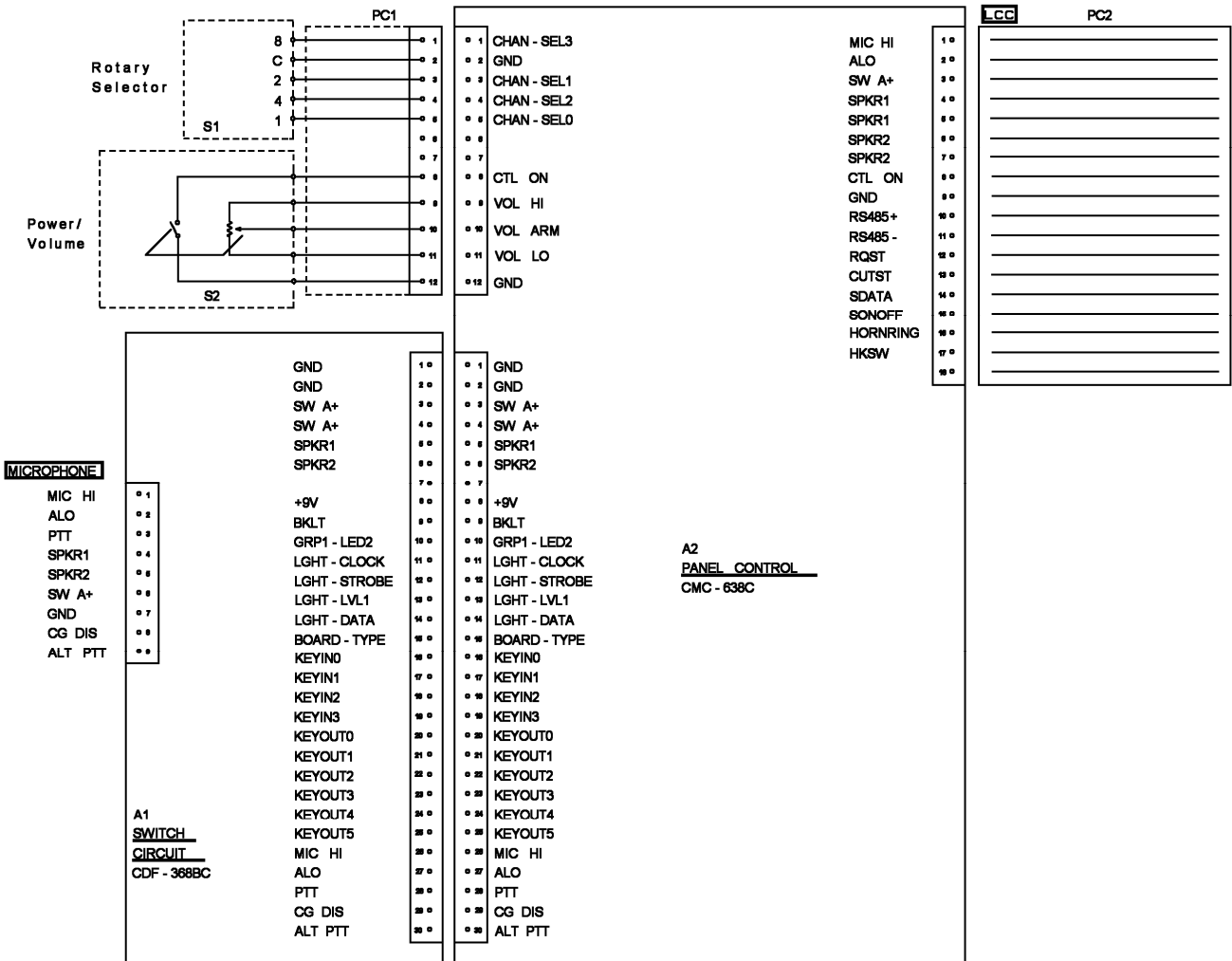
Figure 13-1: Control Unit (Scan Local) (ED00-CMD-556BLC)
