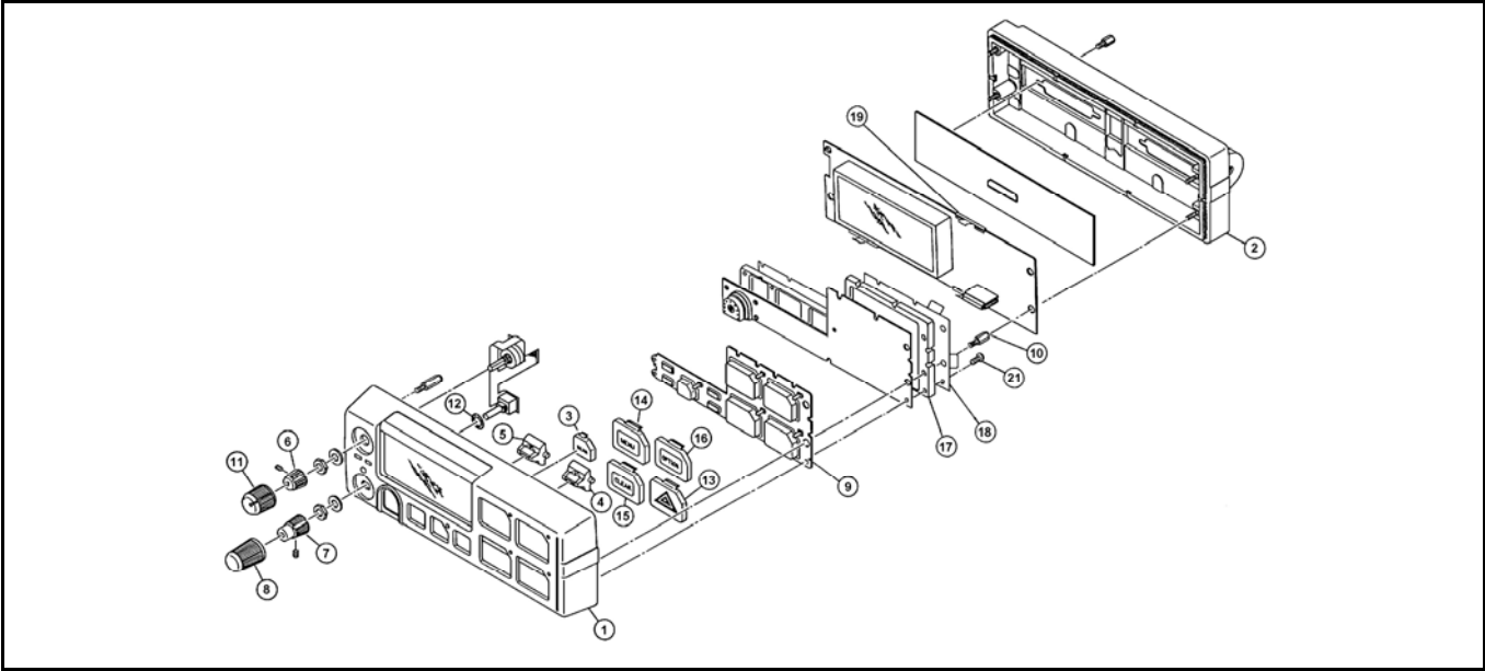
Figure 10-2: Remote Scan Model KRY 101 1632/12 CMC-556 BRC, Sh. 1)
