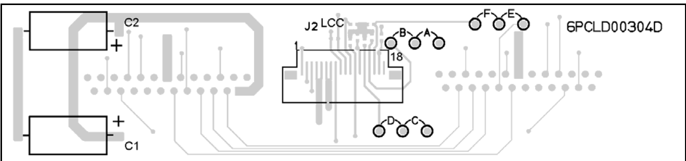
Figure 8-4: Remote Interface Adaptor NQZ-4882C Solder Side
