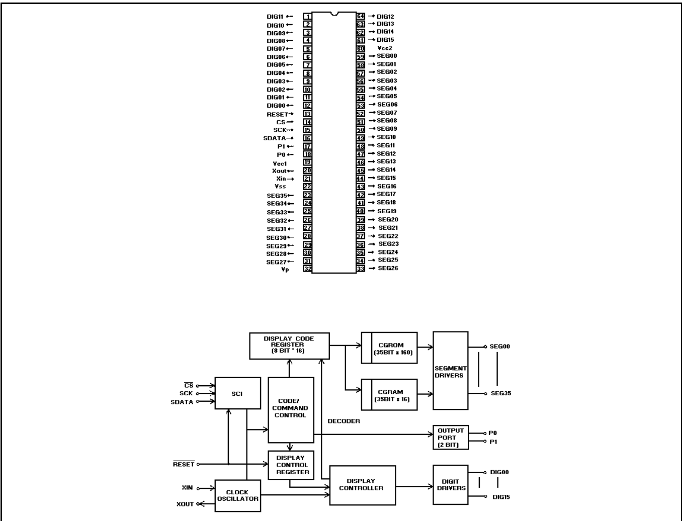
Figure 7-11: IC209 VFC Controller (M66004FP)
