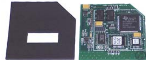
NTM2011102/1 AMPF Module Kit (Pop Filter removes unwanted pops And clicks from a received signal) Includes AMPF Module, Rubber Pad and Ground Strap (not shown)
