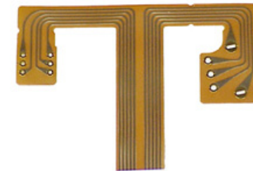
B19/6PCLD00307A Assembly,PCB,Flex Volume Switch
