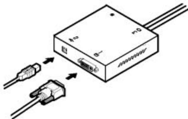
Fig. 9 Connection of the Dual Link signal cable and the converter box
