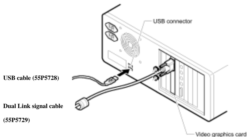
Fig. 10 Connection of the Dual Link signal cable and a graphics card
