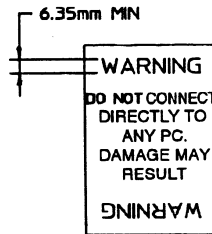
DETAIL FLAG TYPE WARNING LABEL
