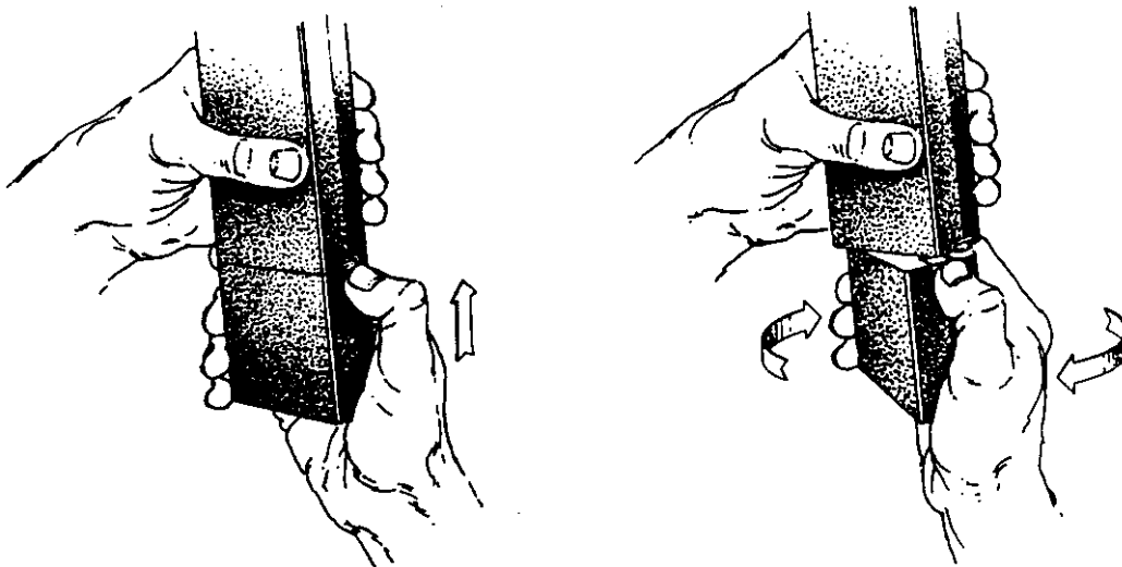
FIGURE 2-1 BATTERY INSTALLATION
