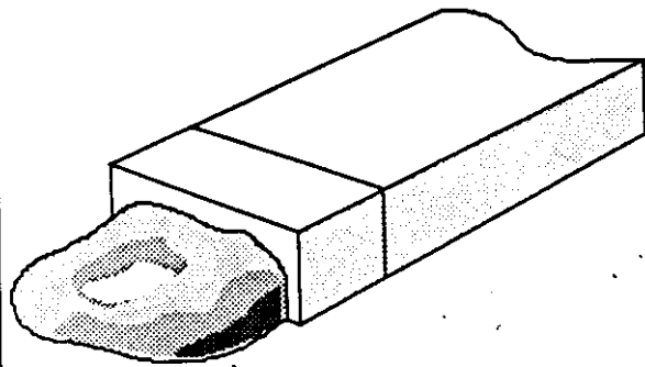
VOID IS LESS THAN 80% OF THE SOLDER WIDTH
